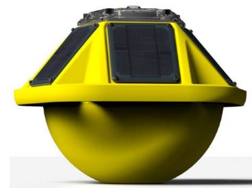
Figure 1: Integral's WaveSpotter V1. Unit height is 13 inches.
