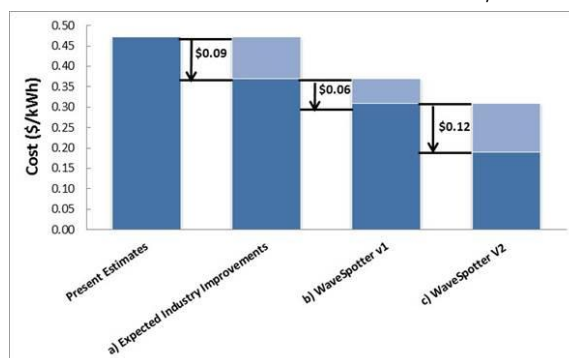
Figure 2: Estimated reductions in the LCOE of wave energy converters. Present estimates 2,3,4 , (a) expected industry improvements (not related to WaveSpotter) 3 (b) estimated benefit of incorporation of WaveSpotter v1 into the WEC array, (c) estimated benefit of incorporation of WaveSpotter v2 into the WEC array.
